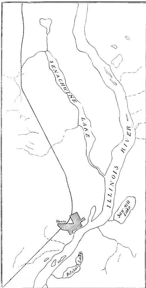
FIG. 9. Map showing lakes on Illinois River flood-plain near Henry. (From Lacon topographic map, U. S. Geol. Surv.)
